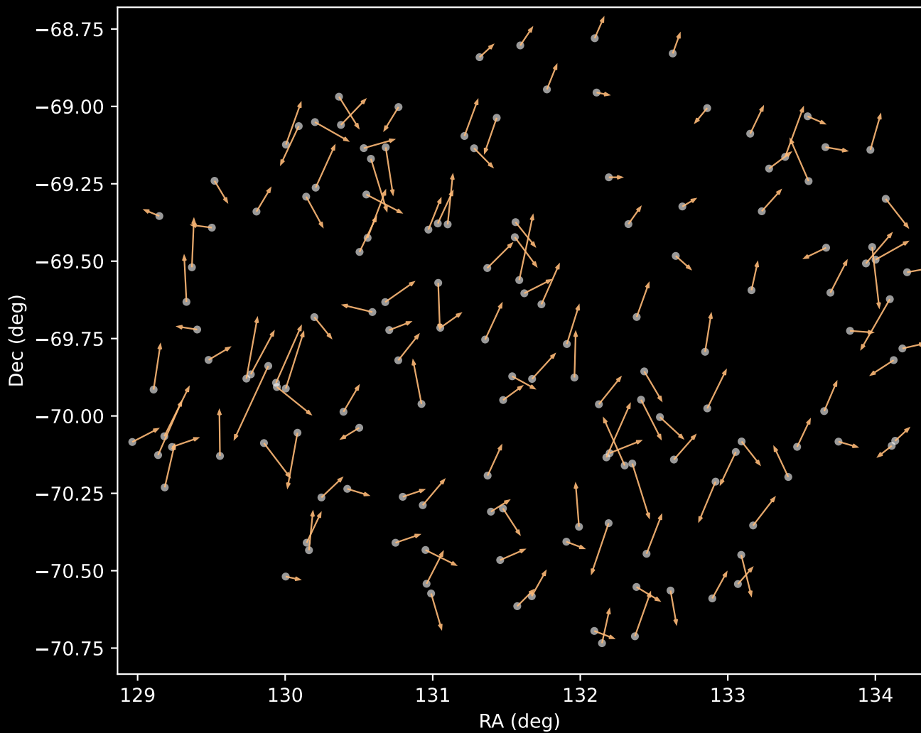
GALAH DR4 Cluster 3 Proper Motion Vectors (n=147)
