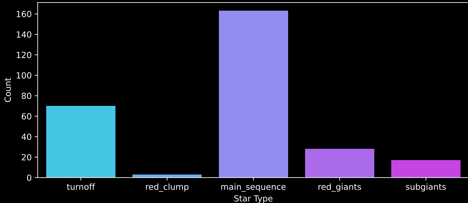
GALAH DR4 Field: [7075] Count plot of Star Type
