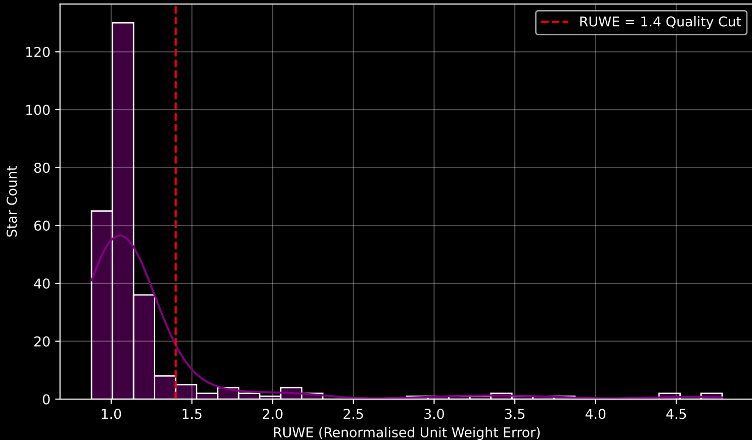
GALAH DR4 Field [7075] RUWE Distribution (n= 272)
