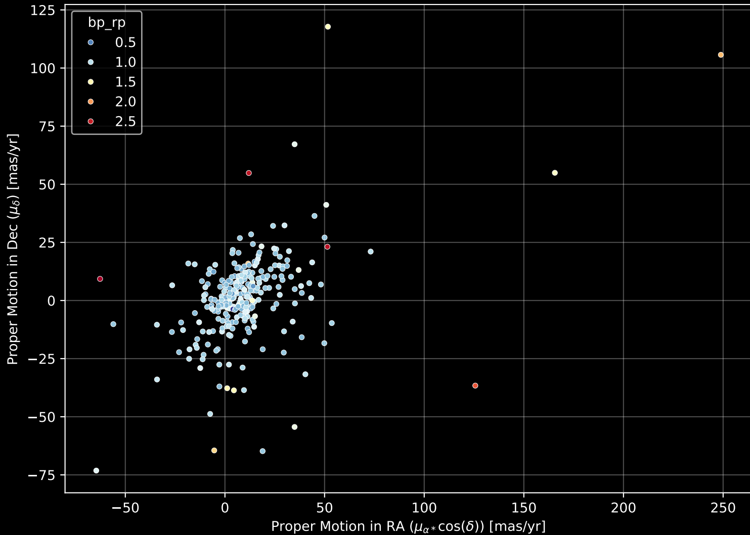
GALAH DR4 Field: [7075] Proper Motion Diagram (n= 281)
