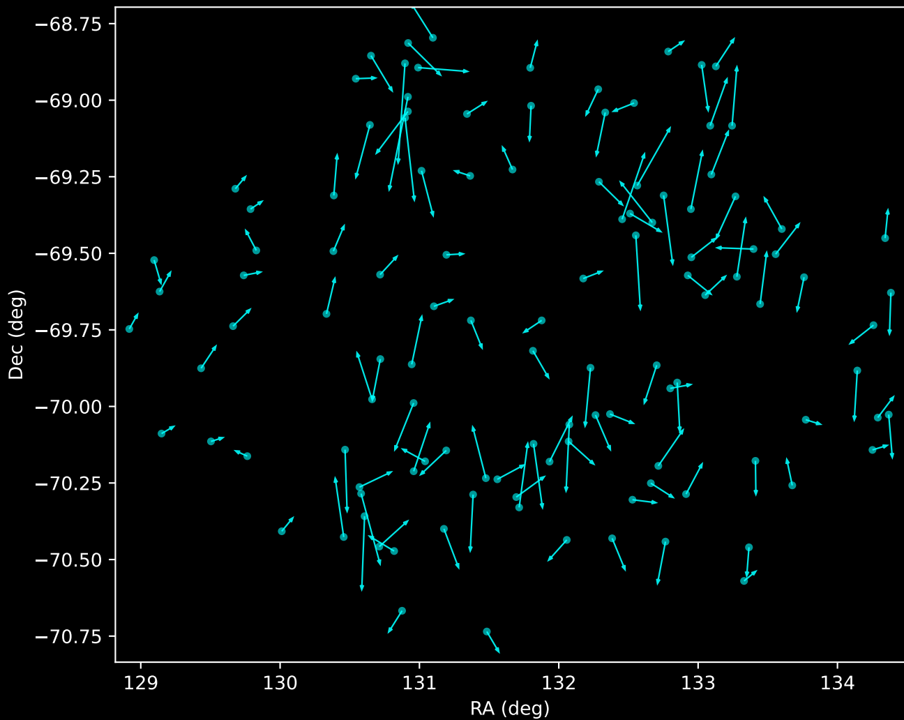
GALAH DR4 Noise Stream Proper Motion Vectors (n=117)
